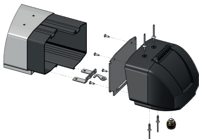
ABS CAP DETAIL
