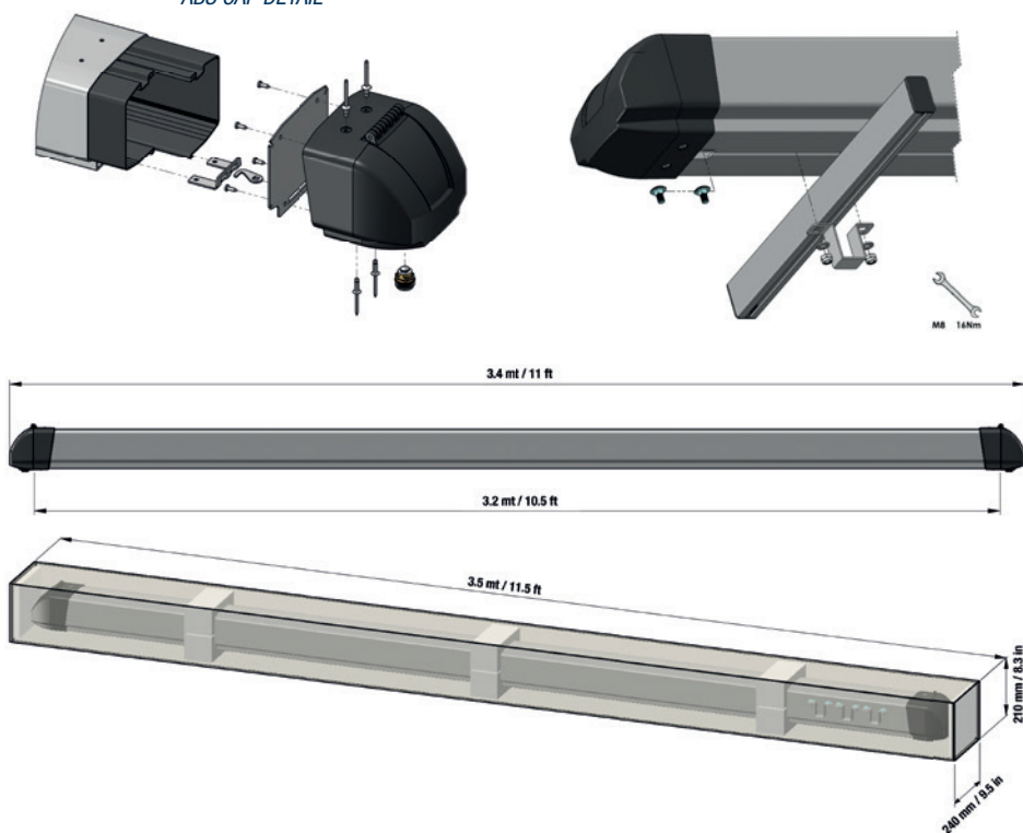
ABS CAP DETAIL
